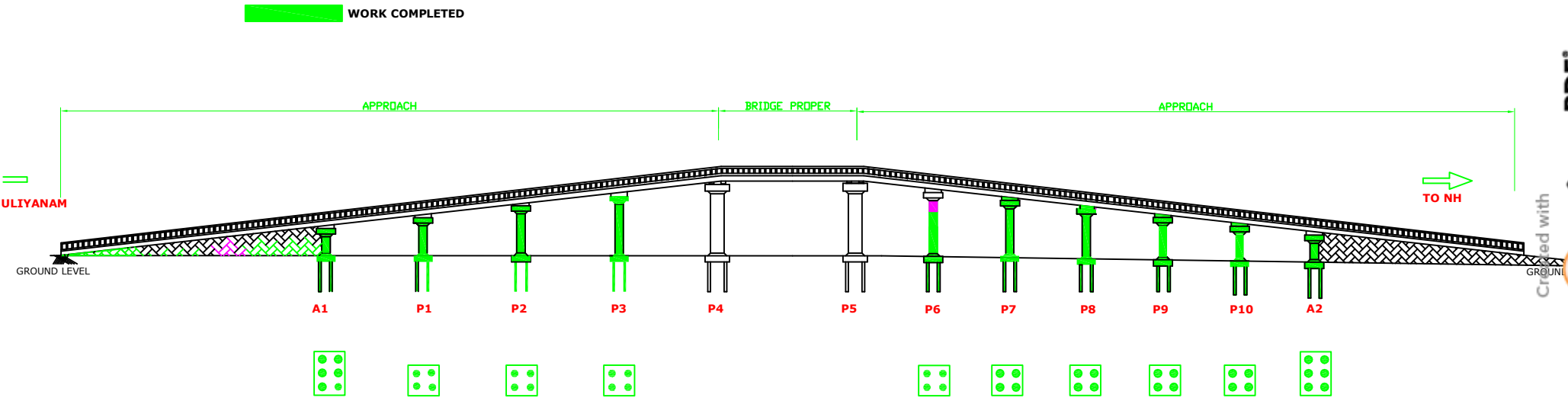
PILE FOUNDATION
